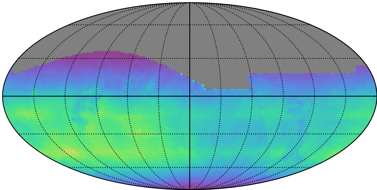
ddf_acor_sf25_lsf40_lsr20_v3.4_10yrs All sky all bands: Normalized Teff
