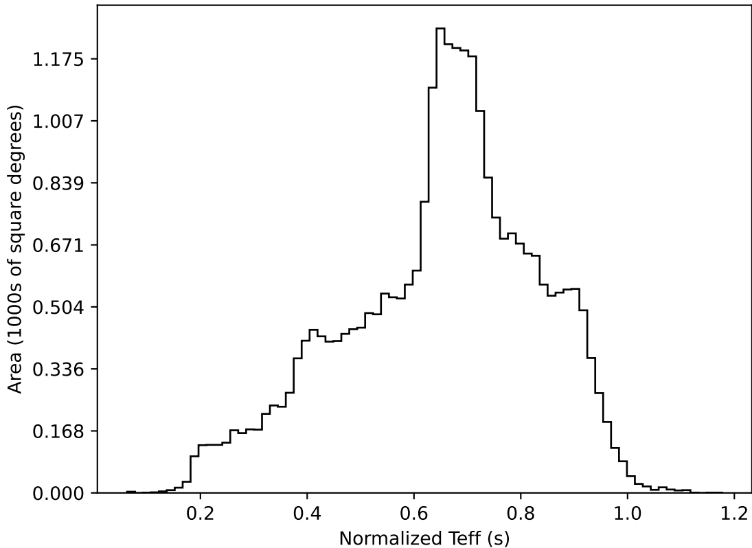
ddf_acor_sf25_lsf40_lsr20_v3.4_10yrs All sky all bands: Normalized Teff
