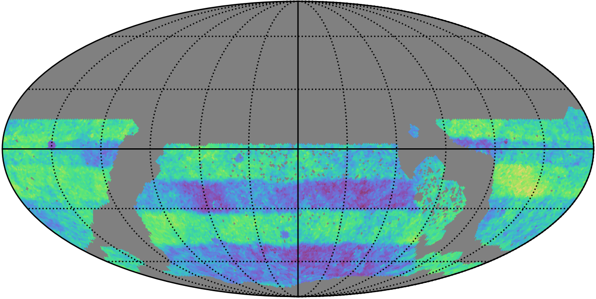
ddf_acor_sf25_lsf40_lsr20_v3.4_10yrs WFD: Normalized Proper Motion Uncert @ 24.0
