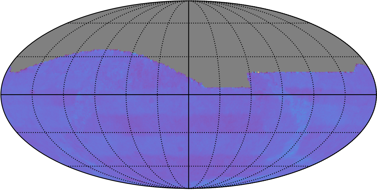
ddf_acor_sf25_lsf40_lsr20_v3.4_10yrs All sky: Normalized Proper Motion Uncert @ 24.0
