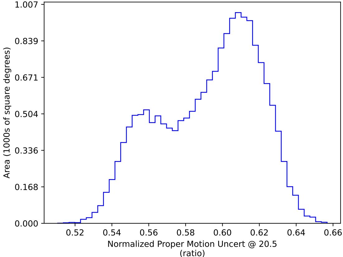
ddf_acor_sf25_lsf40_lsr20_v3.4_10yrs WFD: Normalized Proper Motion Uncert @ 20.5
