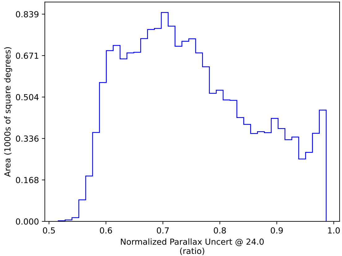
ddf_acor_sf25_lsf40_lsr20_v3.4_10yrs WFD: Normalized Parallax Uncert @ 24.0
