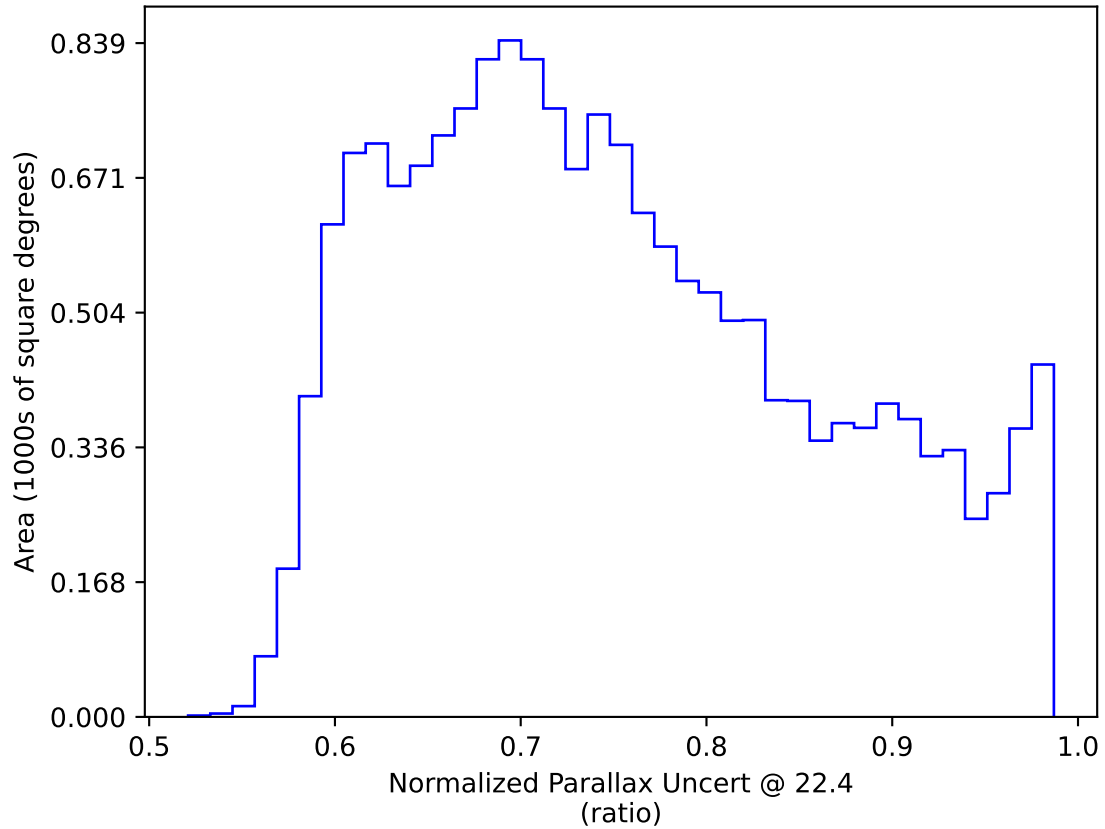
ddf_acor_sf25_lsf40_lsr20_v3.4_10yrs WFD: Normalized Parallax Uncert @ 22.4
