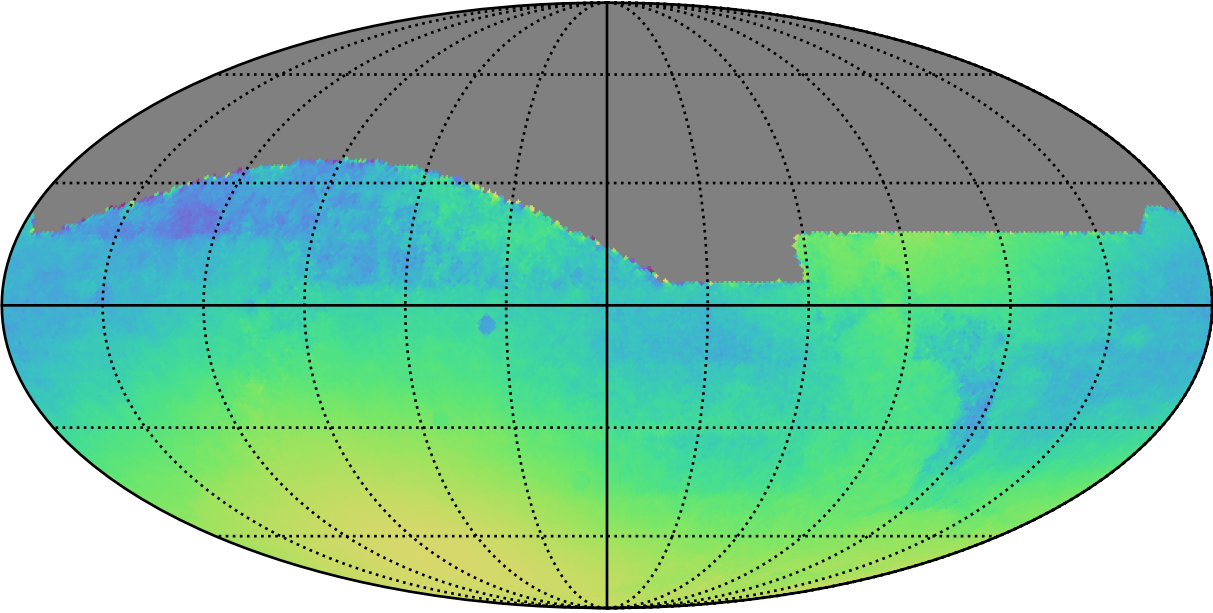
ddf_acor_sf25_lsf40_lsr20_v3.4_10yrs All sky: Normalized Parallax Uncert @ 22.4
