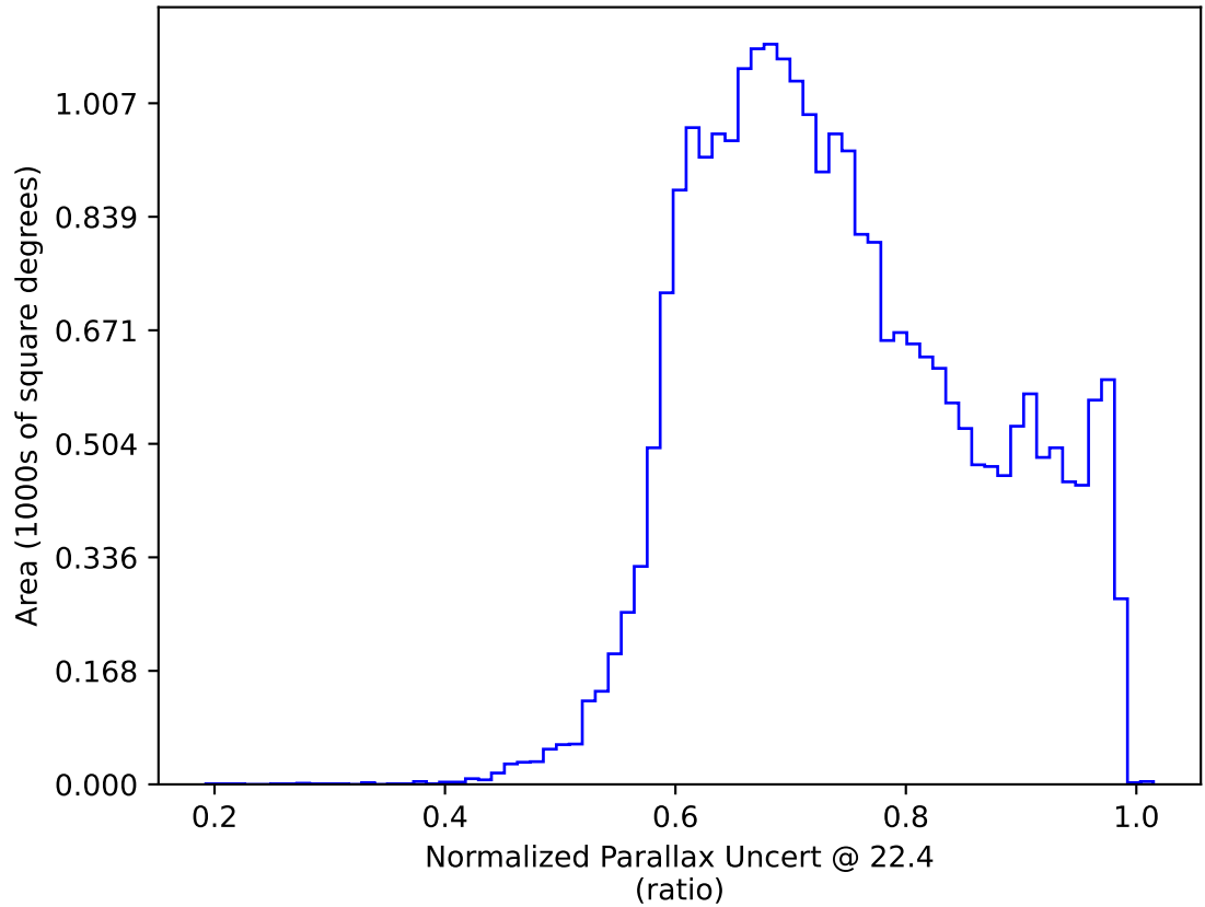
ddf_acor_sf25_lsf40_lsr20_v3.4_10yrs All sky: Normalized Parallax Uncert @ 22.4
