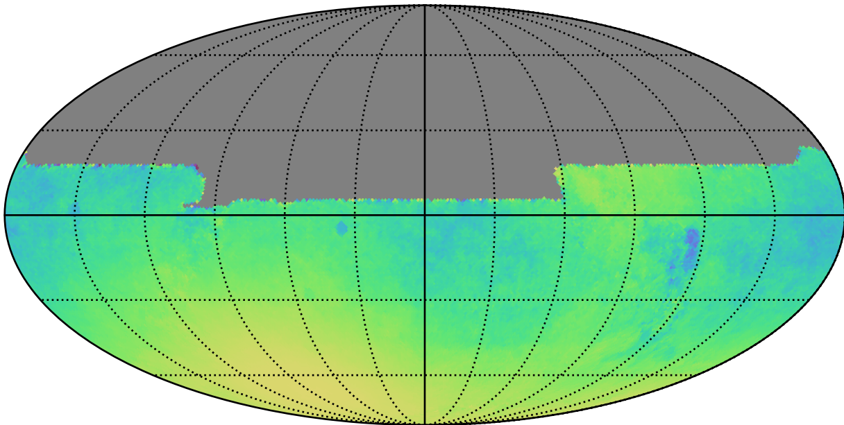
ddf_acor_sf25_lsf40_lsr20_v3.4_10yrs All sky y band only: Normalized Parallax Uncert @ 21.3
