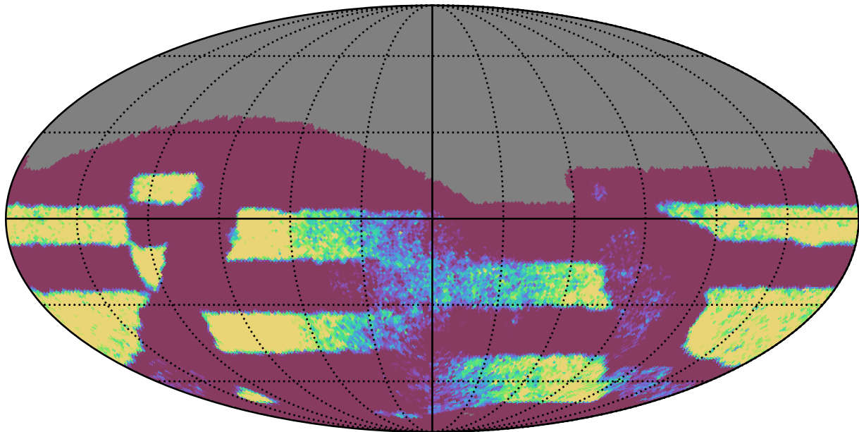
ddf_acor_sf25_lsf40_lsr20_v3.4_10yrs Yr 3-4 all bands: NVisits
