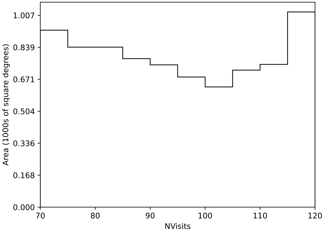
ddf_acor_sf25_lsf40_lsr20_v3.4_10yrs Yr 3-4 all bands: NVisits
