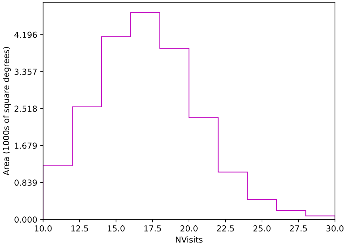
ddf_acor_sf25_lsf40_lsr20_v3.4_10yrs Yr 1 z band: NVisits
