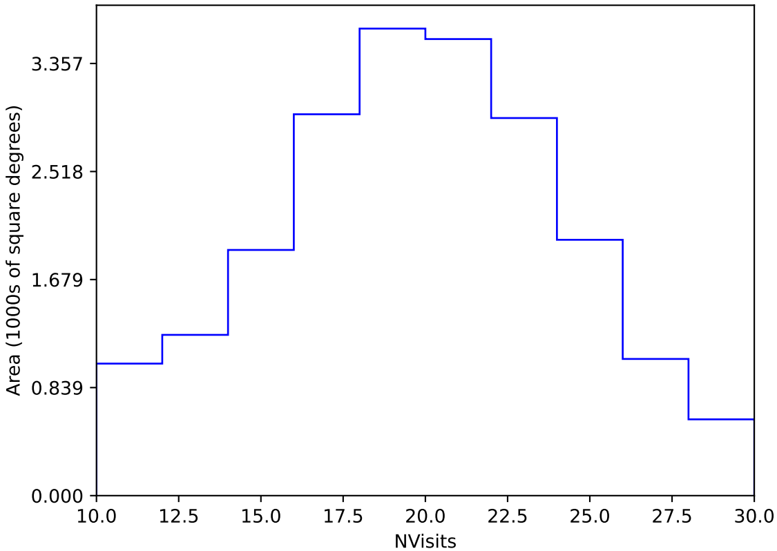
ddf_acor_sf25_lsf40_lsr20_v3.4_10yrs Yr 1 y band: NVisits
