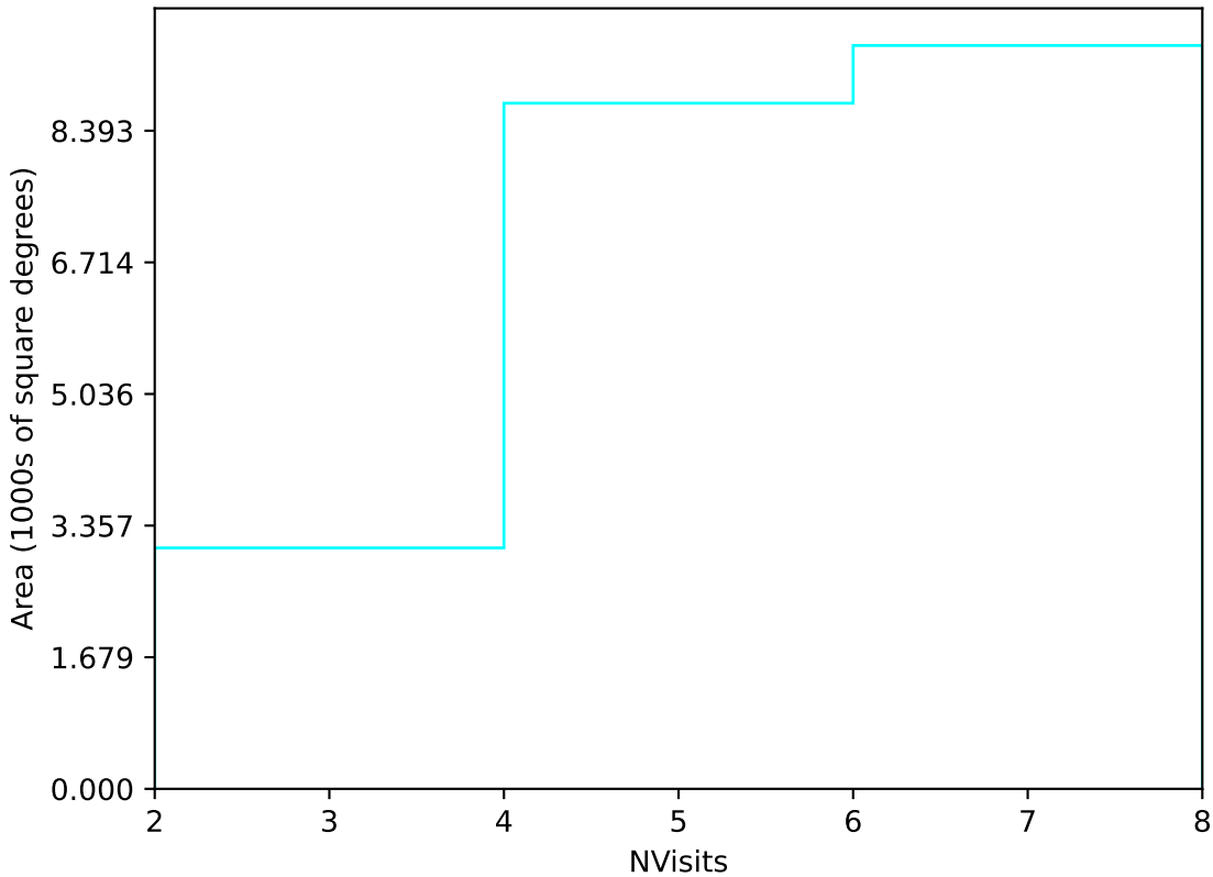
ddf_acor_sf25_lsf40_lsr20_v3.4_10yrs Yr 1 u band: NVisits
