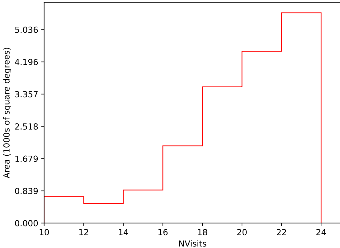
ddf_acor_sf25_lsf40_lsr20_v3.4_10yrs Yr 1 i band: NVisits
