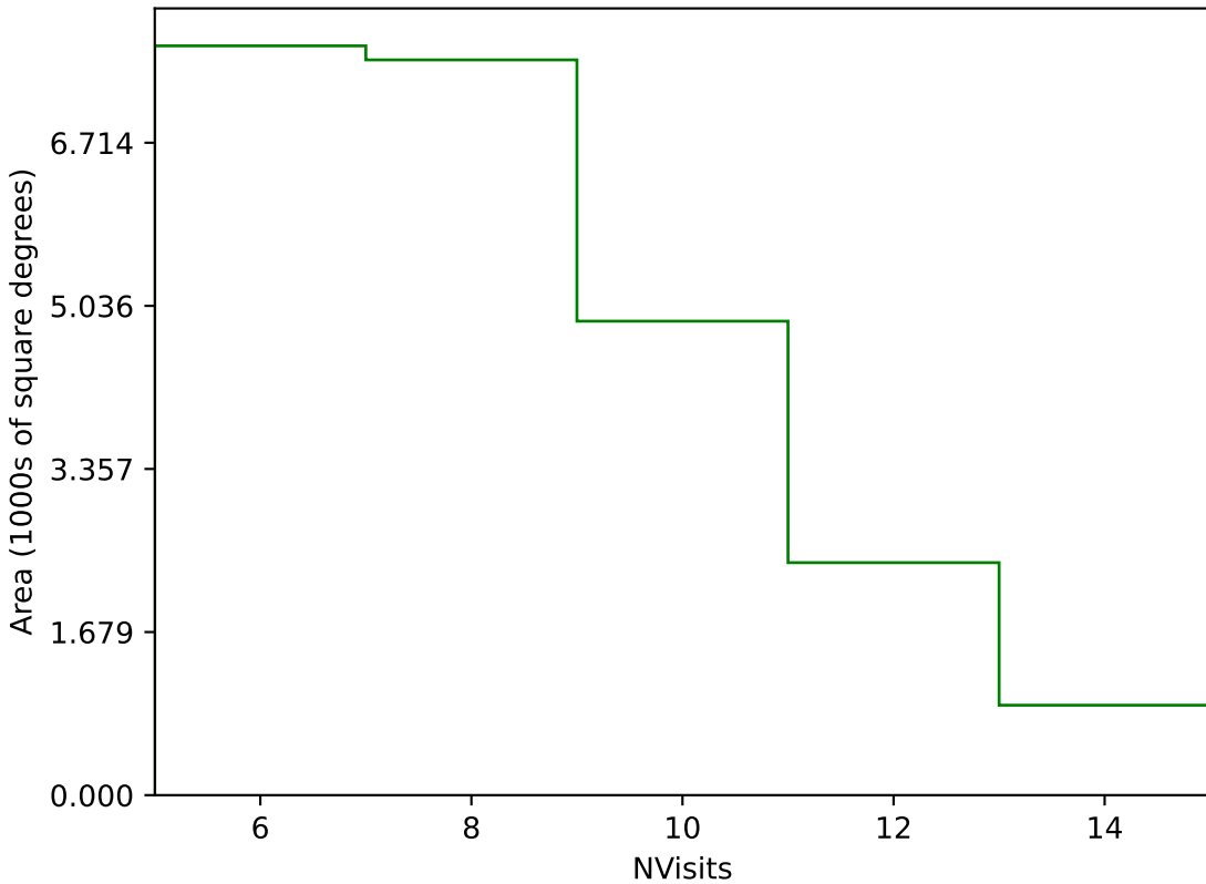
ddf_acor_sf25_lsf40_lsr20_v3.4_10yrs Yr 1 g band: NVisits
