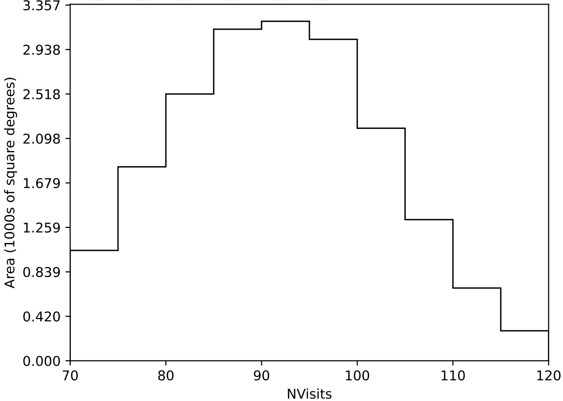
ddf_acor_sf25_lsf40_lsr20_v3.4_10yrs Yr 1 all bands: NVisits
