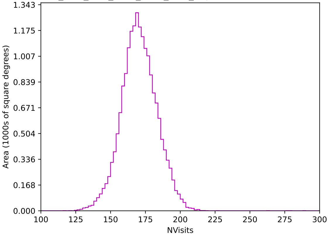
ddf_acor_sf25_lsf40_lsr20_v3.4_10yrs WFD z band: NVisits
