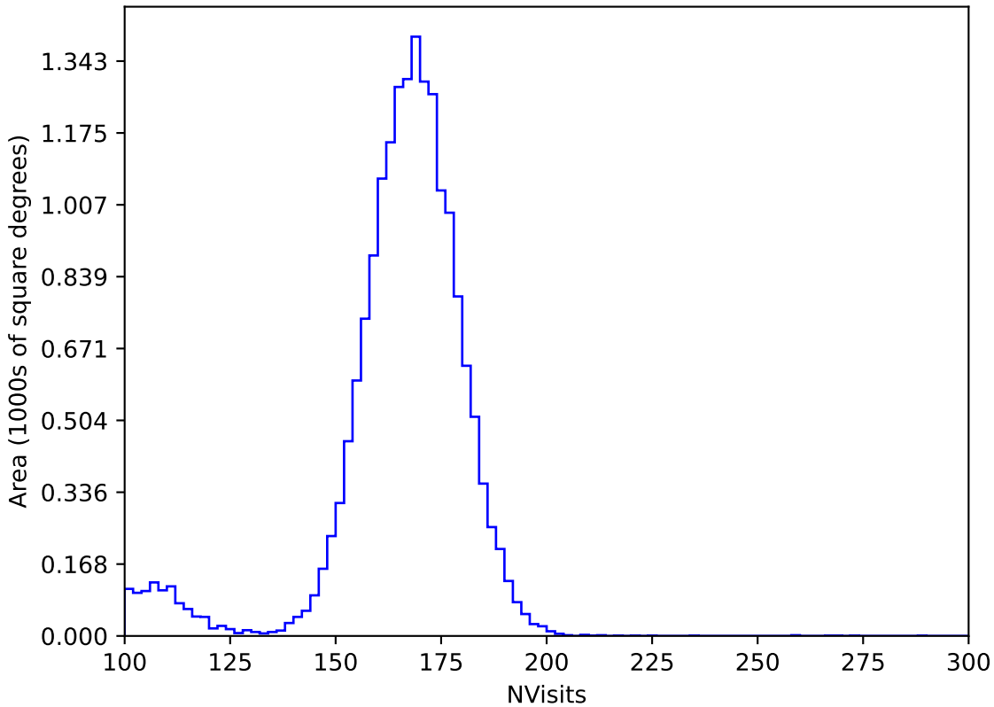
ddf_acor_sf25_lsf40_lsr20_v3.4_10yrs WFD y band: NVisits
