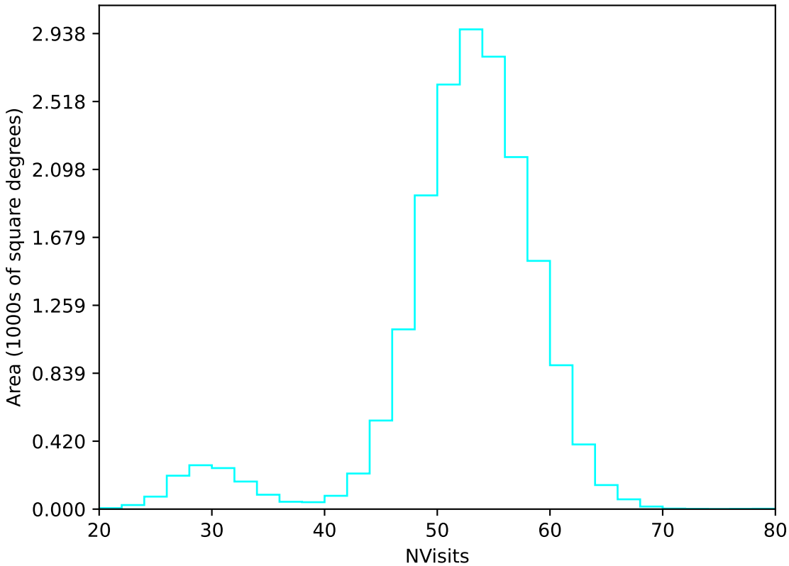
ddf_acor_sf25_lsf40_lsr20_v3.4_10yrs WFD u band: NVisits
