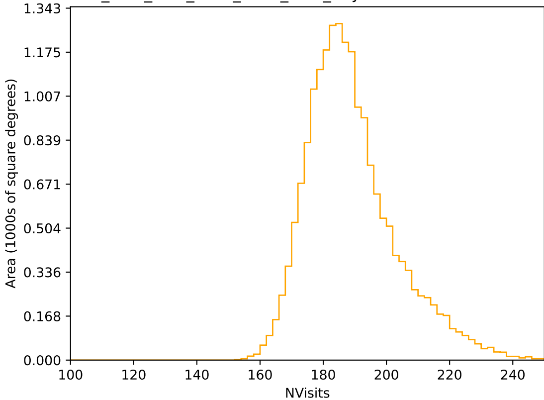
ddf_acor_sf25_lsf40_lsr20_v3.4_10yrs WFD r band: NVisits
