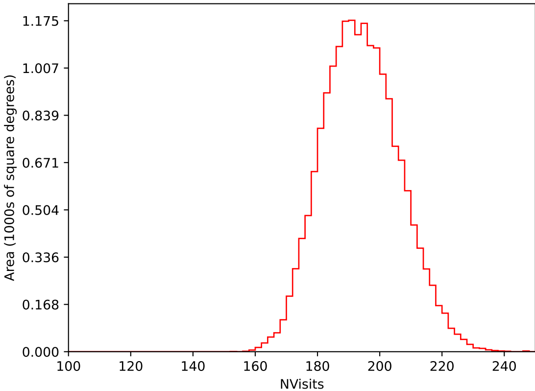
ddf_acor_sf25_lsf40_lsr20_v3.4_10yrs WFD i band: NVisits
