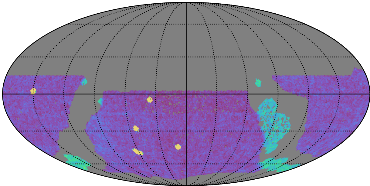
ddf_acor_sf25_lsf40_lsr20_v3.4_10yrs WFD g band: NVisits
