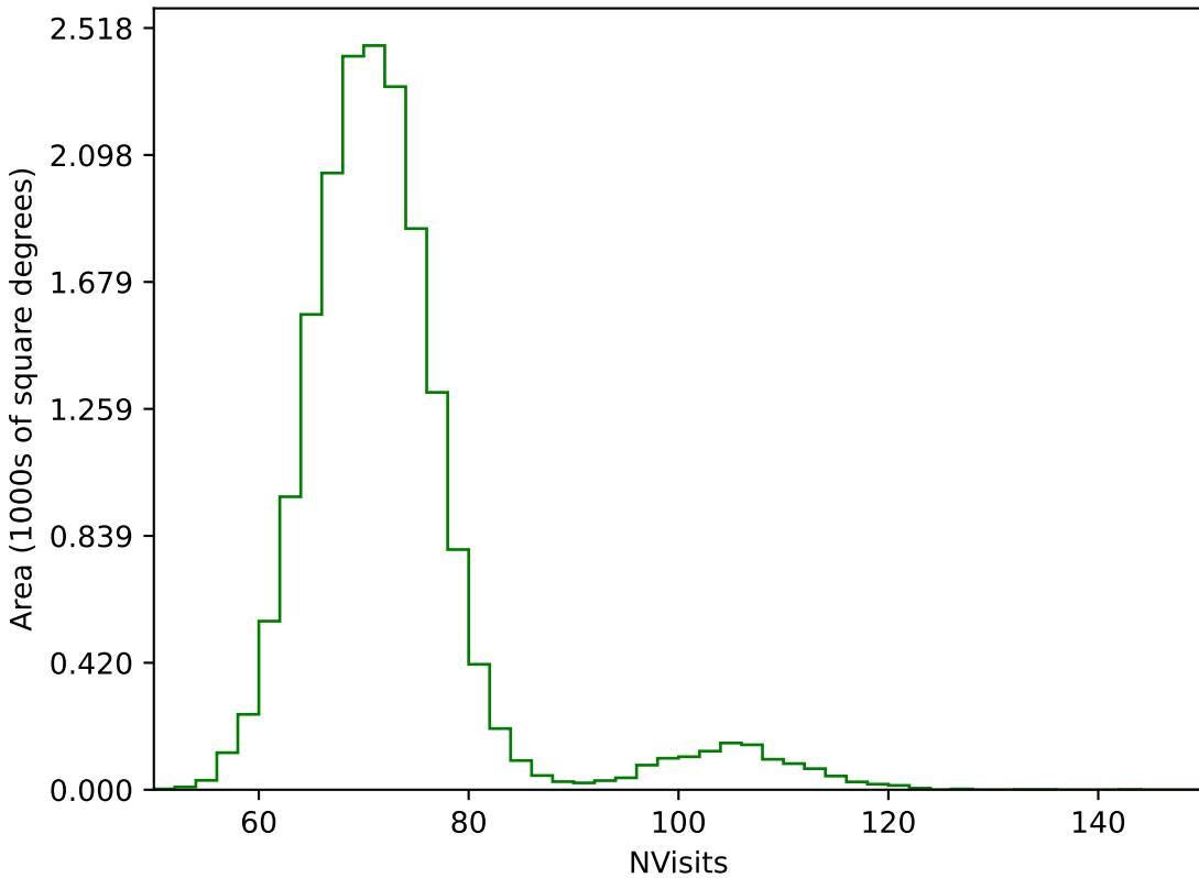
ddf_acor_sf25_lsf40_lsr20_v3.4_10yrs WFD g band: NVisits
