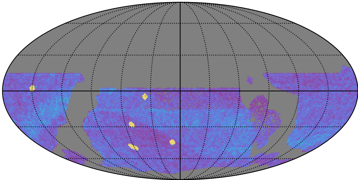
ddf_acor_sf25_lsf40_lsr20_v3.4_10yrs WFD all bands: NVisits
