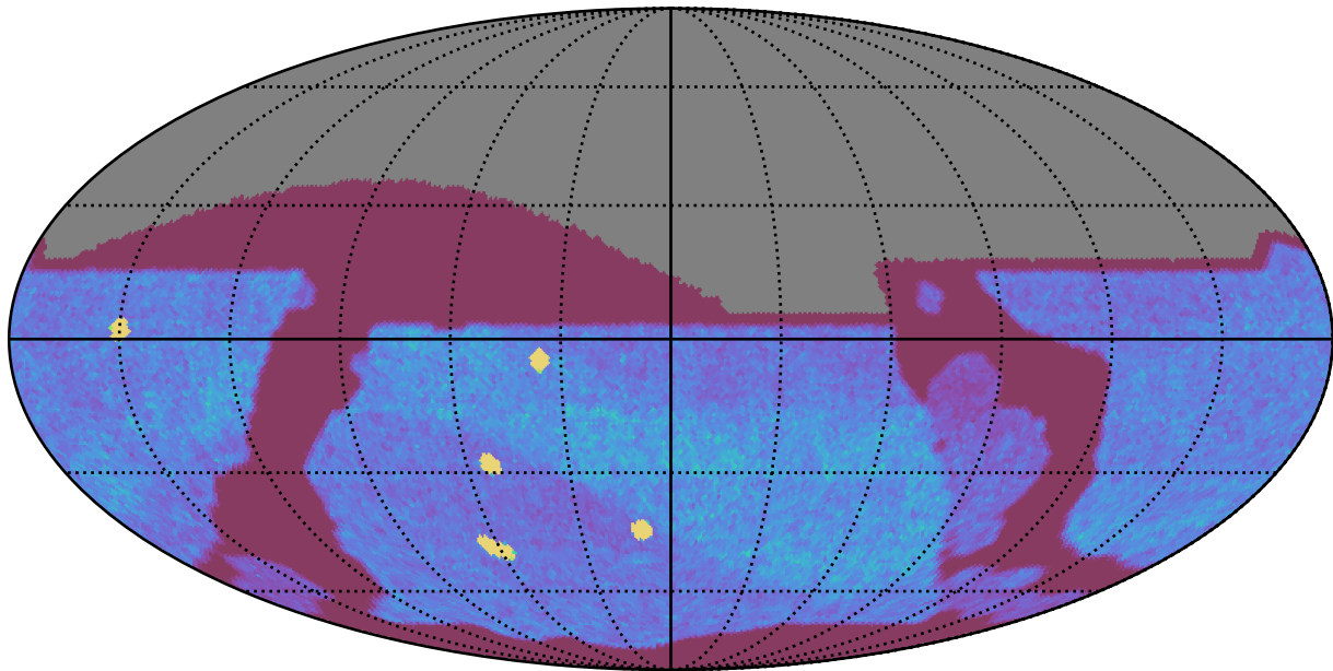
ddf_acor_sf25_lsf40_lsr20_v3.4_10yrs All sky z band: NVisits
