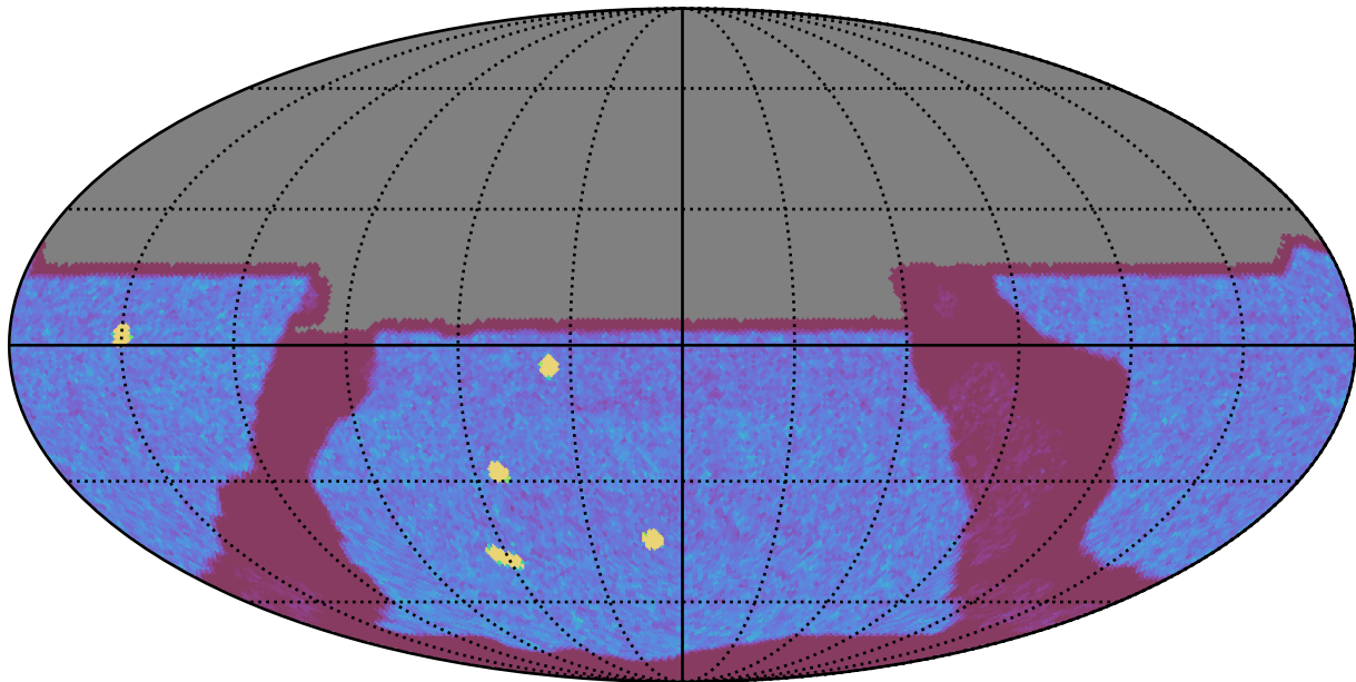
ddf_acor_sf25_lsf40_lsr20_v3.4_10yrs All sky y band: NVisits
