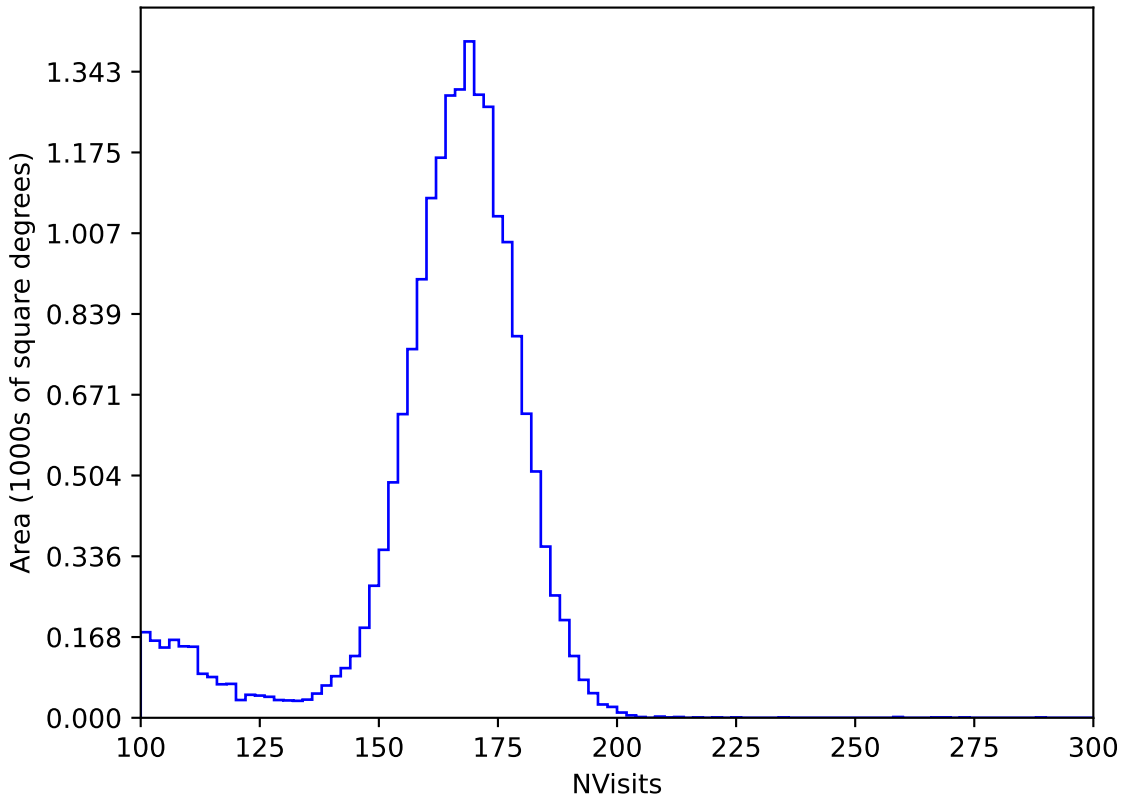
ddf_acor_sf25_lsf40_lsr20_v3.4_10yrs All sky y band: NVisits
