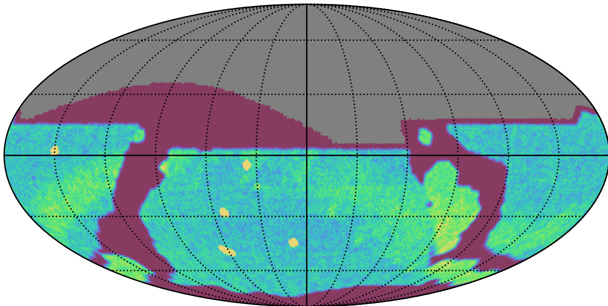
ddf_acor_sf25_lsf40_lsr20_v3.4_10yrs All sky r band: NVisits
