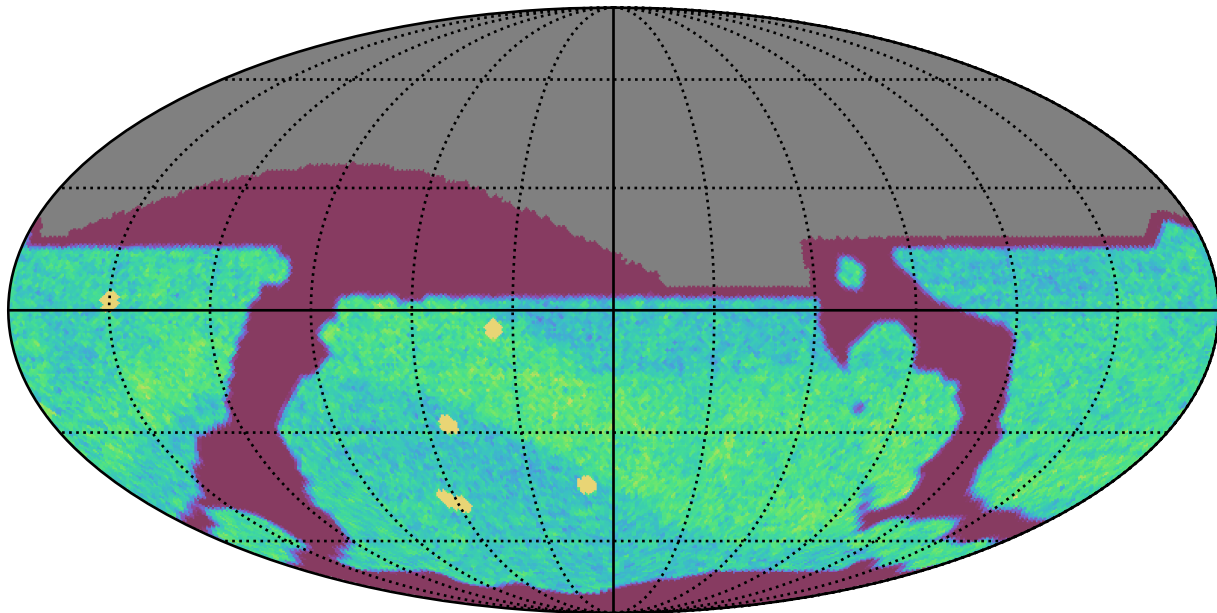
ddf_acor_sf25_lsf40_lsr20_v3.4_10yrs All sky i band: NVisits
