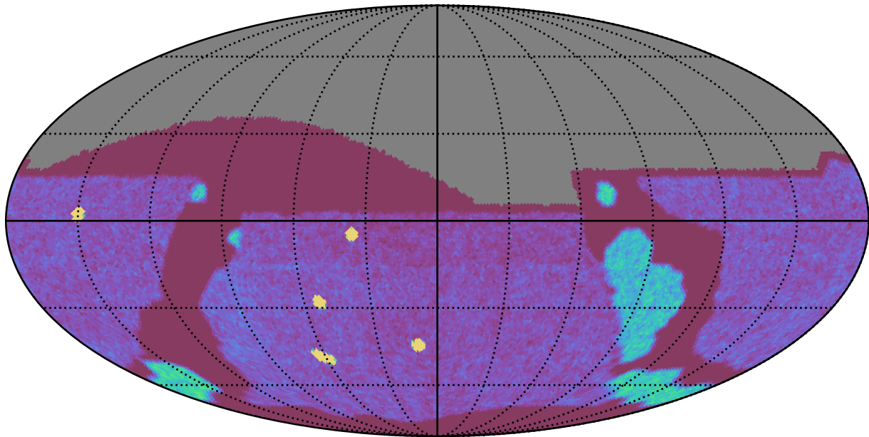
ddf_acor_sf25_lsf40_lsr20_v3.4_10yrs All sky g band: NVisits
