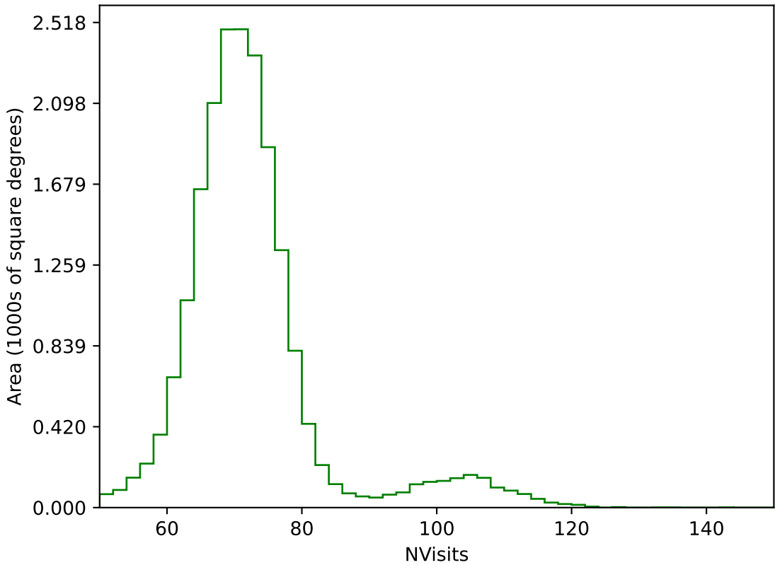
ddf_acor_sf25_lsf40_lsr20_v3.4_10yrs All sky g band: NVisits
