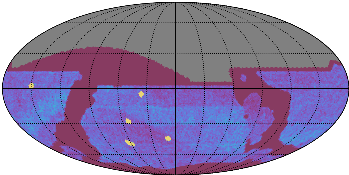
ddf_acor_sf25_lsf40_lsr20_v3.4_10yrs All sky all bands: NVisits
