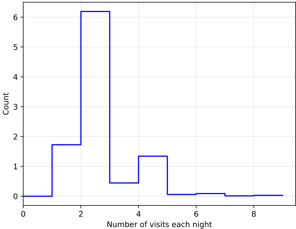
ddf_acor_sf25_lsf40_lsr20_v3.4_10yrs All sky: NVisitsPerNight 1e6
