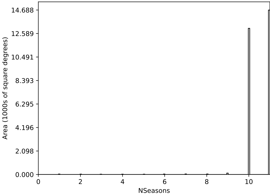
ddf_acor_sf25_lsf40_lsr20_v3.4_10yrs All sky all bands: NSeasons
