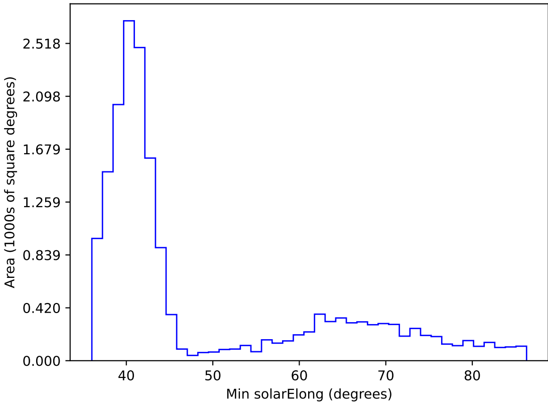
ddf_acor_sf25_lsf40_lsr20_v3.4_10yrs WFD z band: Min solarElong
