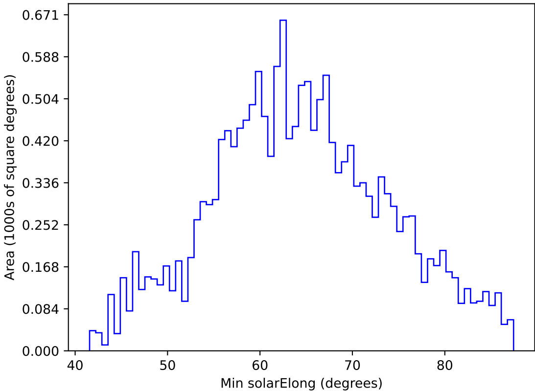
ddf_acor_sf25_lsf40_lsr20_v3.4_10yrs WFD y band: Min solarElong
