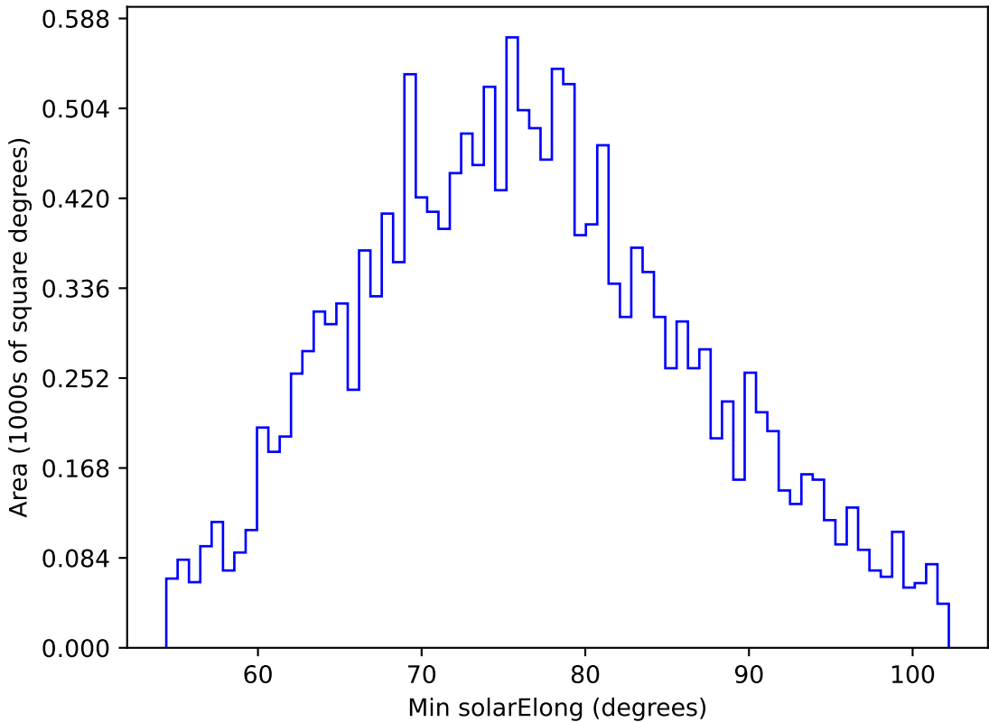
ddf_acor_sf25_lsf40_lsr20_v3.4_10yrs WFD u band: Min solarElong
