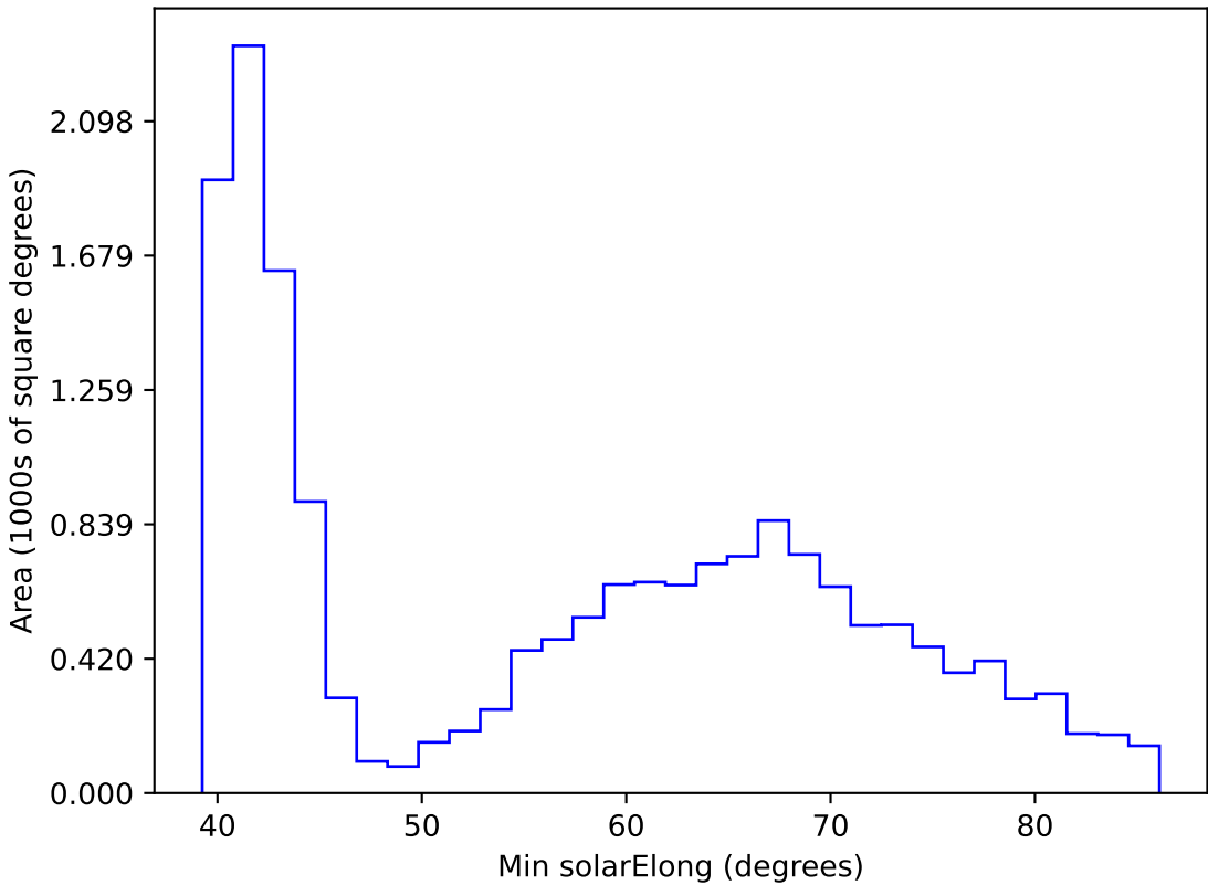
ddf_acor_sf25_lsf40_lsr20_v3.4_10yrs WFD r band: Min solarElong
