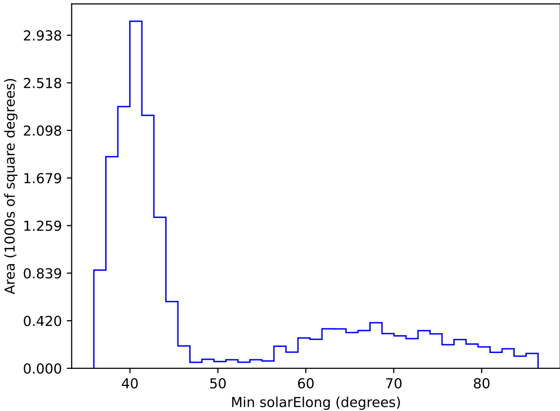
ddf_acor_sf25_lsf40_lsr20_v3.4_10yrs WFD i band: Min solarElong
