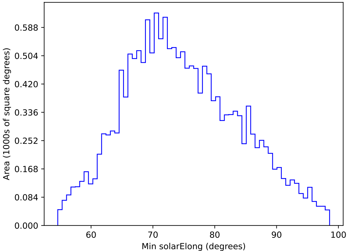
ddf_acor_sf25_lsf40_lsr20_v3.4_10yrs WFD g band: Min solarElong
