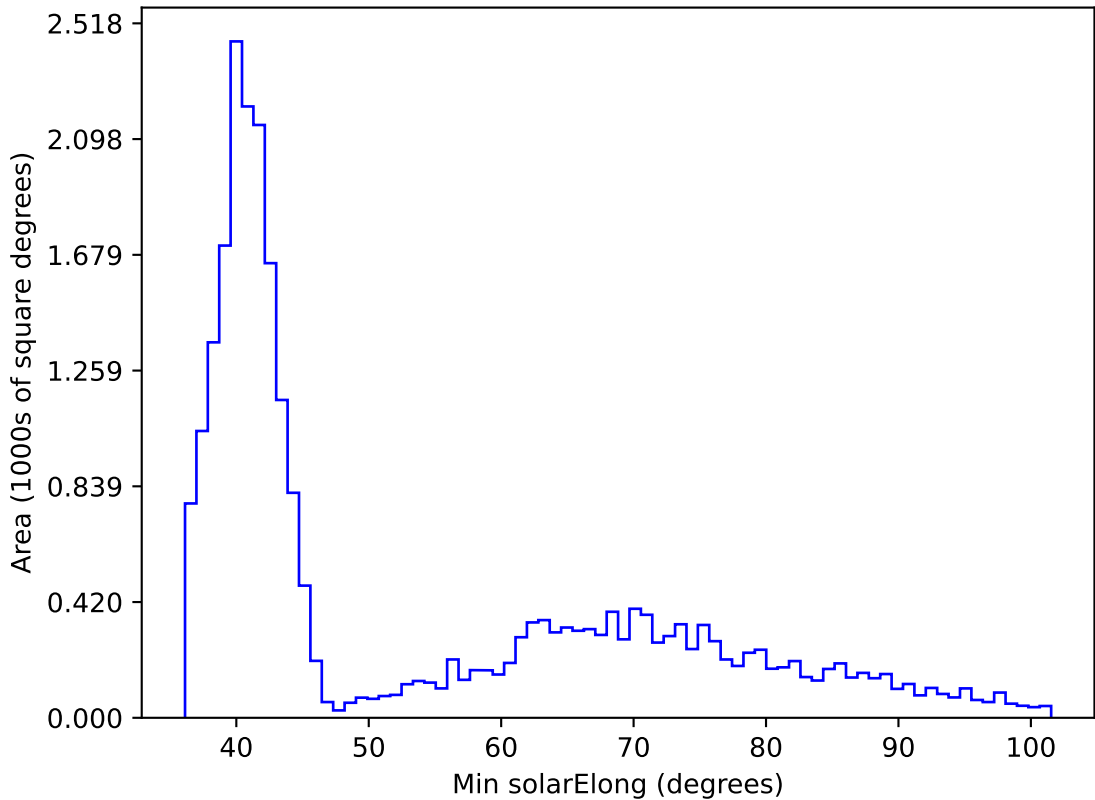
ddf_acor_sf25_lsf40_lsr20_v3.4_10yrs All sky z band: Min solarElong
