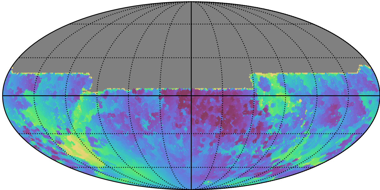
ddf_acor_sf25_lsf40_lsr20_v3.4_10yrs All sky y band: Min solarElong
