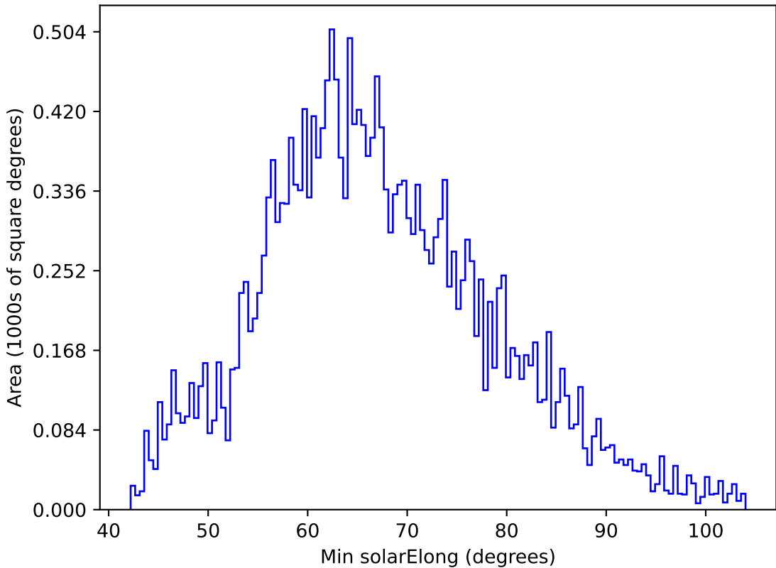
ddf_acor_sf25_lsf40_lsr20_v3.4_10yrs All sky y band: Min solarElong
