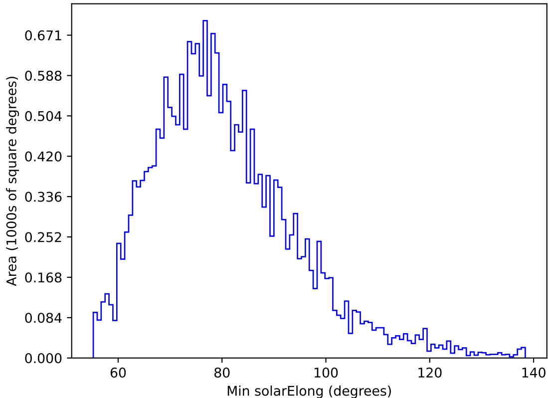
ddf_acor_sf25_lsf40_lsr20_v3.4_10yrs All sky u band: Min solarElong
