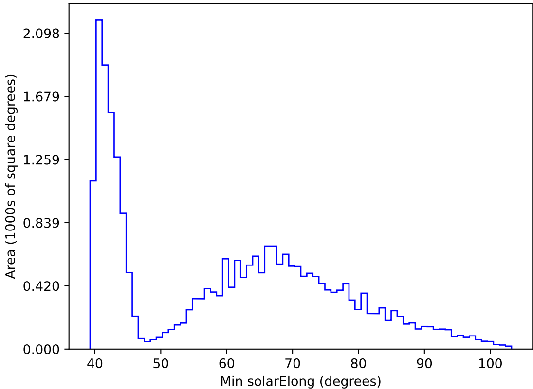
ddf_acor_sf25_lsf40_lsr20_v3.4_10yrs All sky r band: Min solarElong
