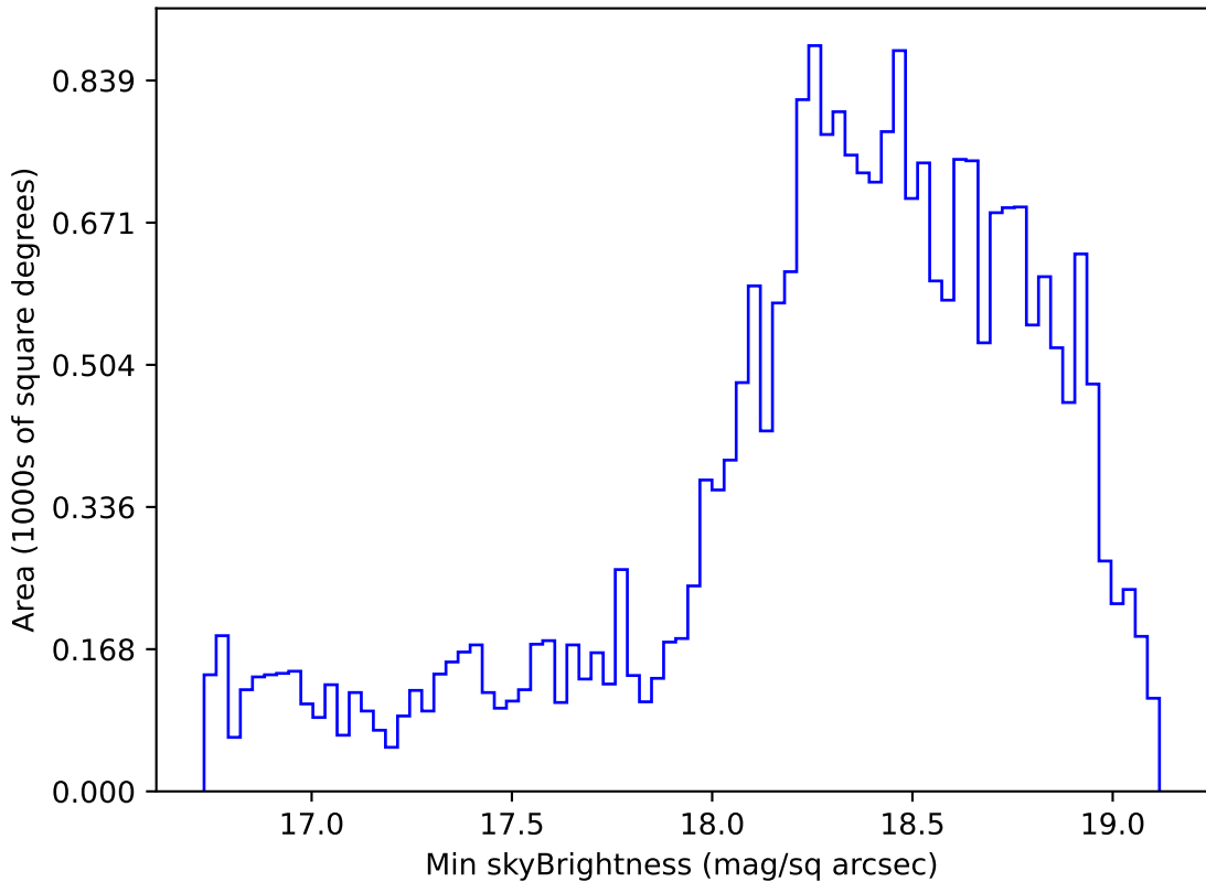
ddf_acor_sf25_lsf40_lsr20_v3.4_10yrs Yr 1 z band: Min skyBrightness
