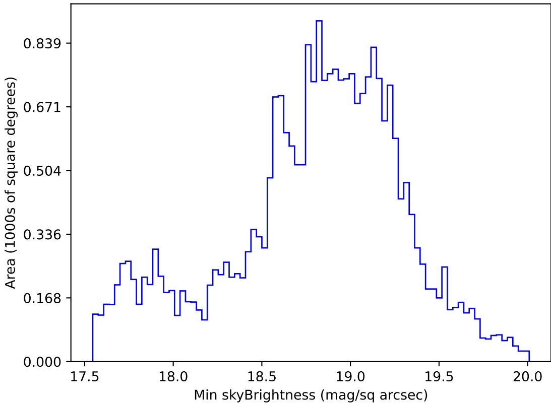
ddf_acor_sf25_lsf40_lsr20_v3.4_10yrs Yr 1 i band: Min skyBrightness
