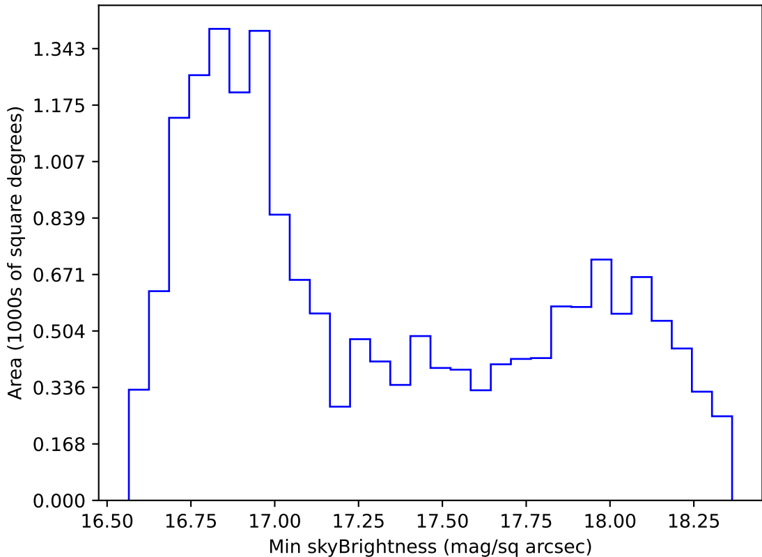
ddf_acor_sf25_lsf40_lsr20_v3.4_10yrs WFD z band: Min skyBrightness
